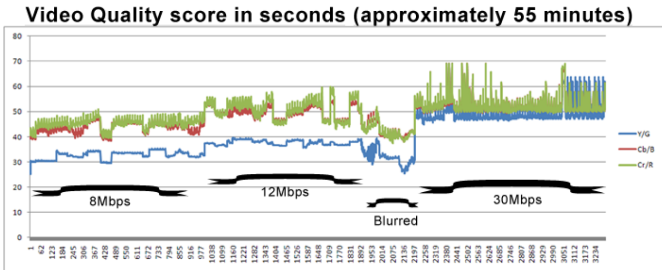
Figure 8: Video Quality Over Time
